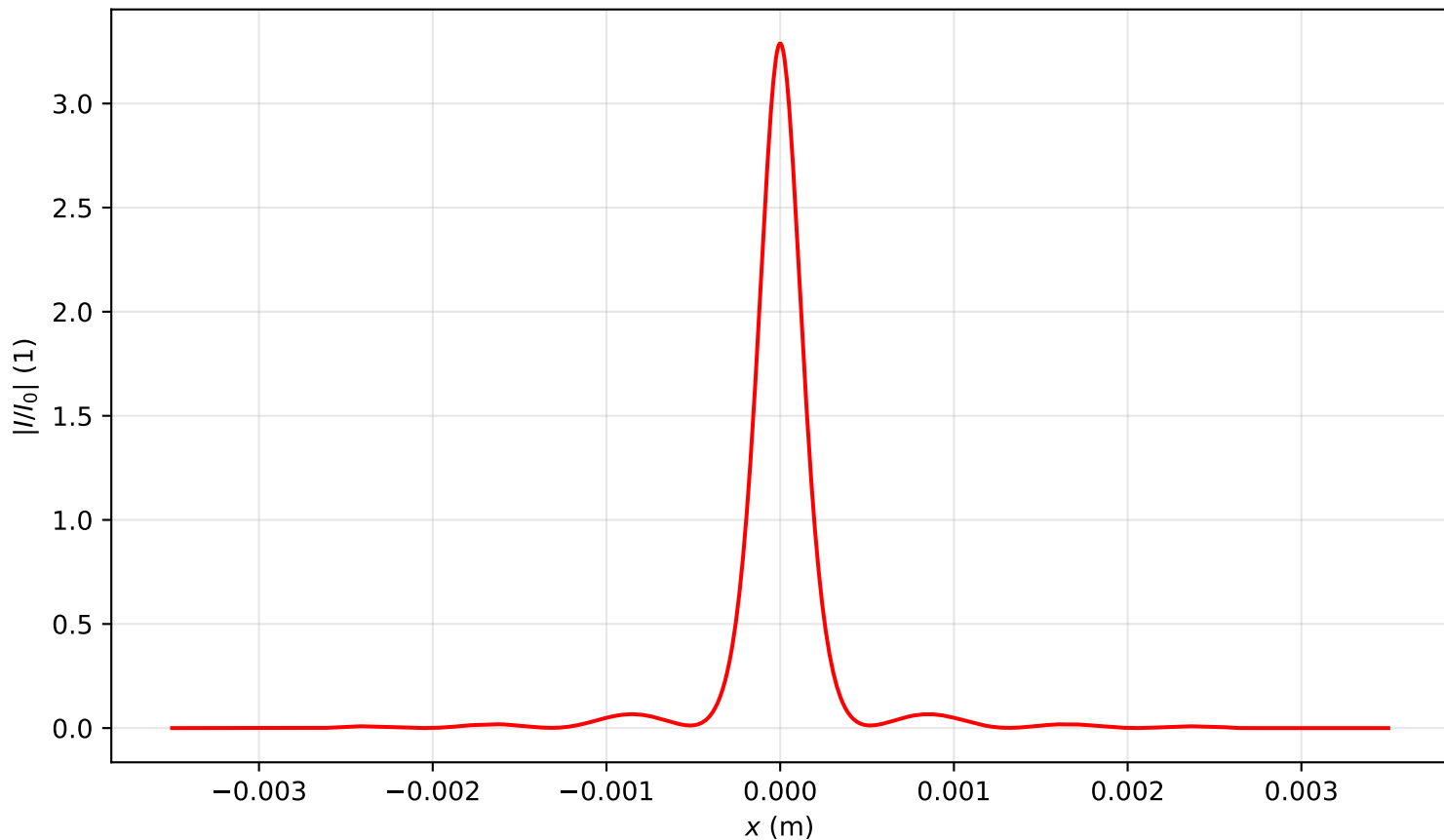
Intensity profile I(x, y = 0, z = 0.637)/I_0 , \text{Pin}=1.0\text{Pcr} , artificial time
